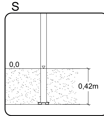
S Sunken Foundation 8105443 8105451
